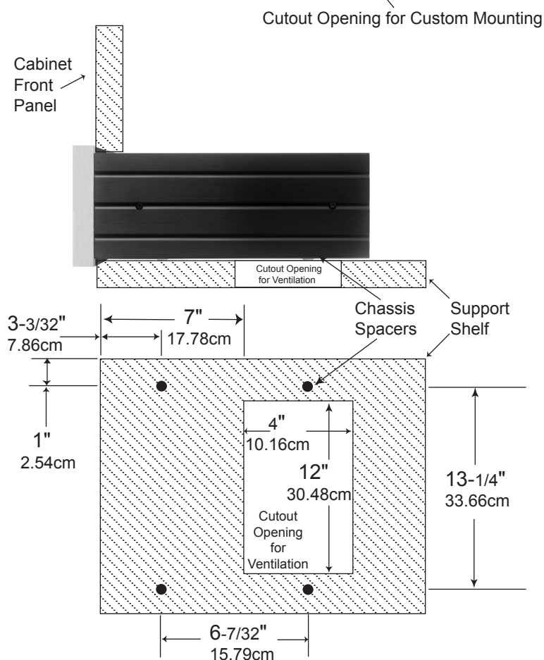
MDA1000 Bottom View in Custom Cabinet
