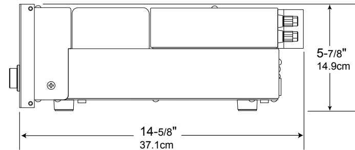
Side Views of the MXA80 Loudspeaker
