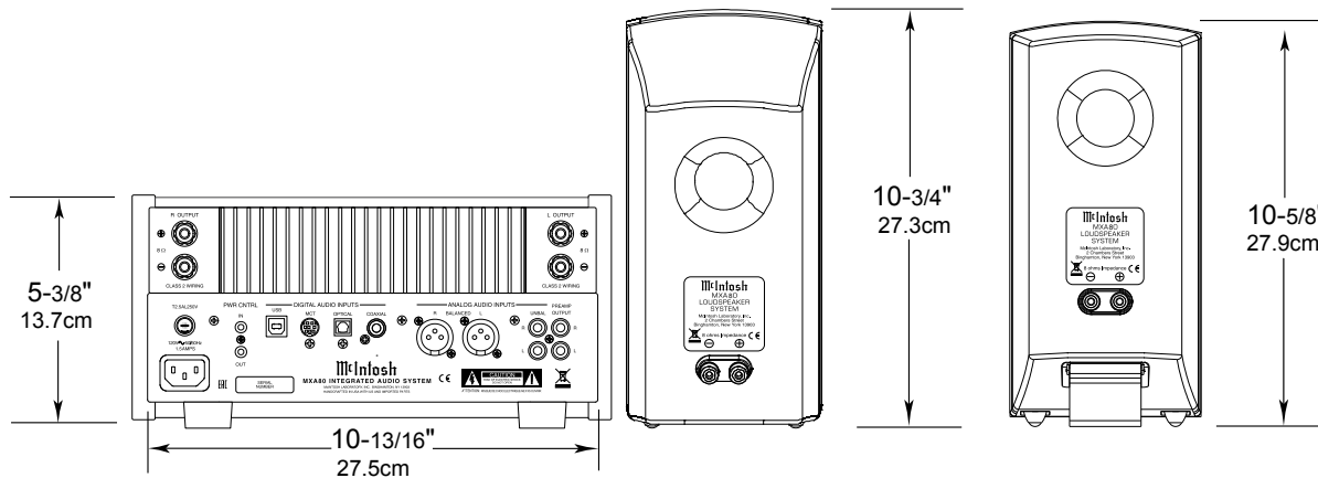
Rear View of the MXA80
