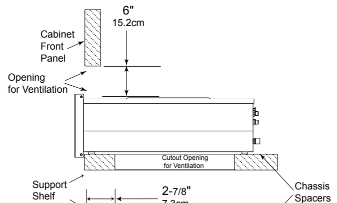
C1100T Side View in Custom Cabinet
