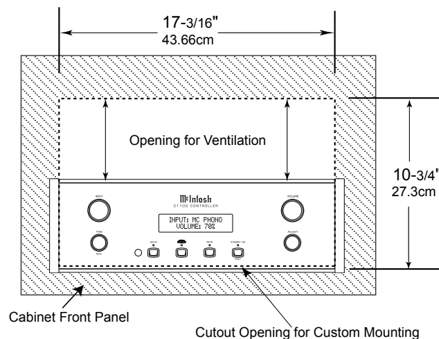
C1100C Front Panel Custom Cabinet Cutout
