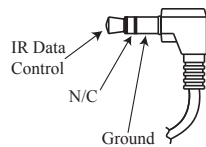
Figure 06– IR 3.5mm connector
