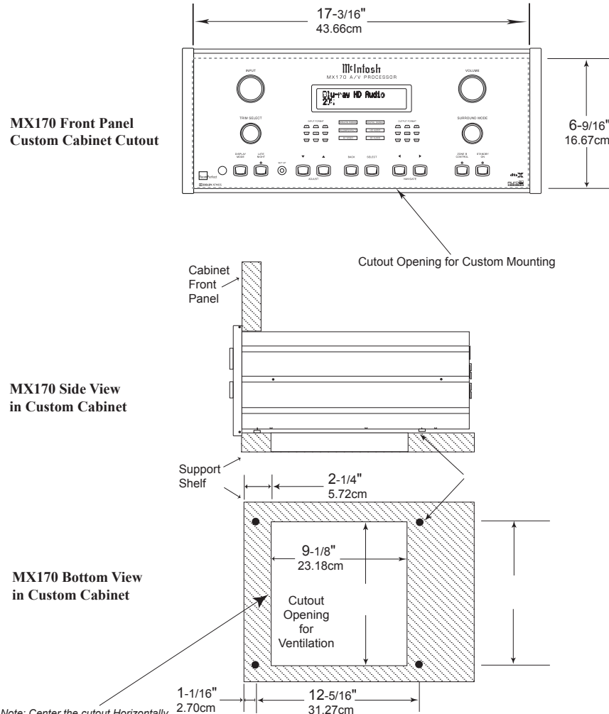
Figure 02– Custom cutout dimensions
