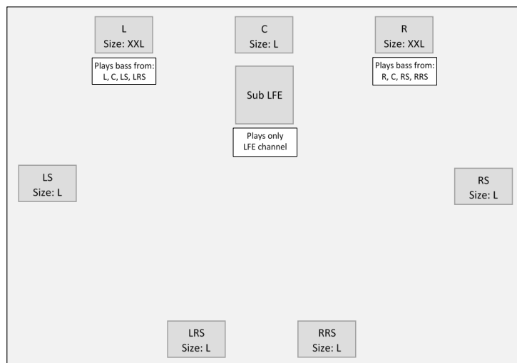
Figure 15– 7.1.4 LFE Sub, Front XXL Speakers
