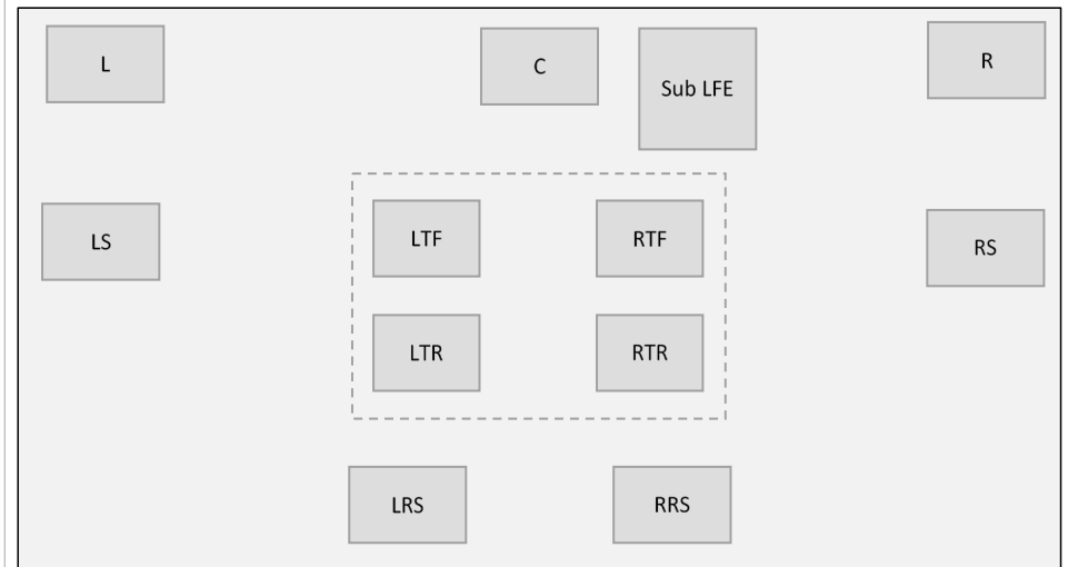
Figure 13– Dolby Atmos Example: 7.1.4
