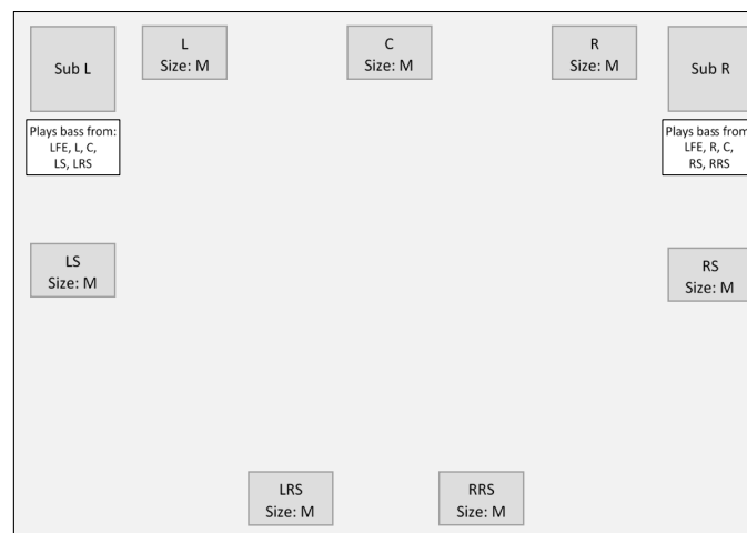
Figure 16– 7.1.4 Front Subs
