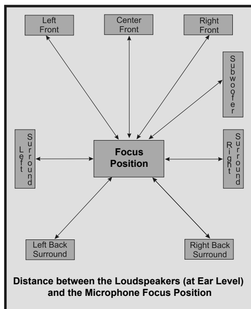
Figure 18– RoomPerfect™ Focus Position
