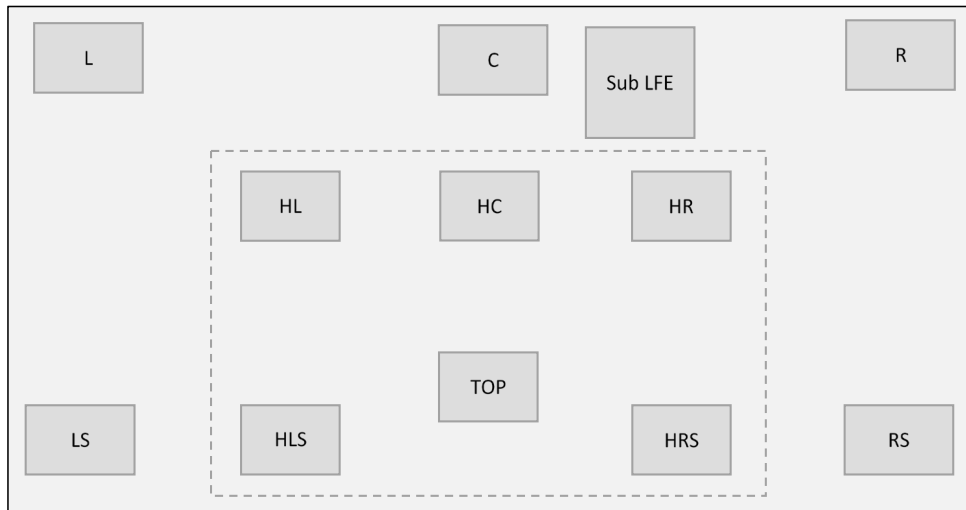
Figure 12– Auro-3D example: 11.1
