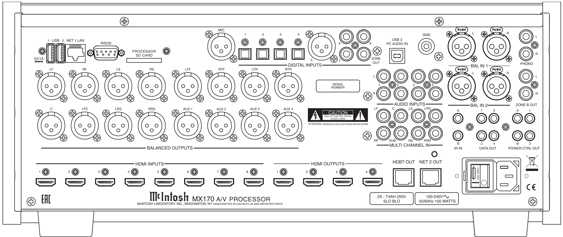
Figure 04– MX170 Rear View
