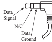
Figure 10– Power control (trigger) mini plug
