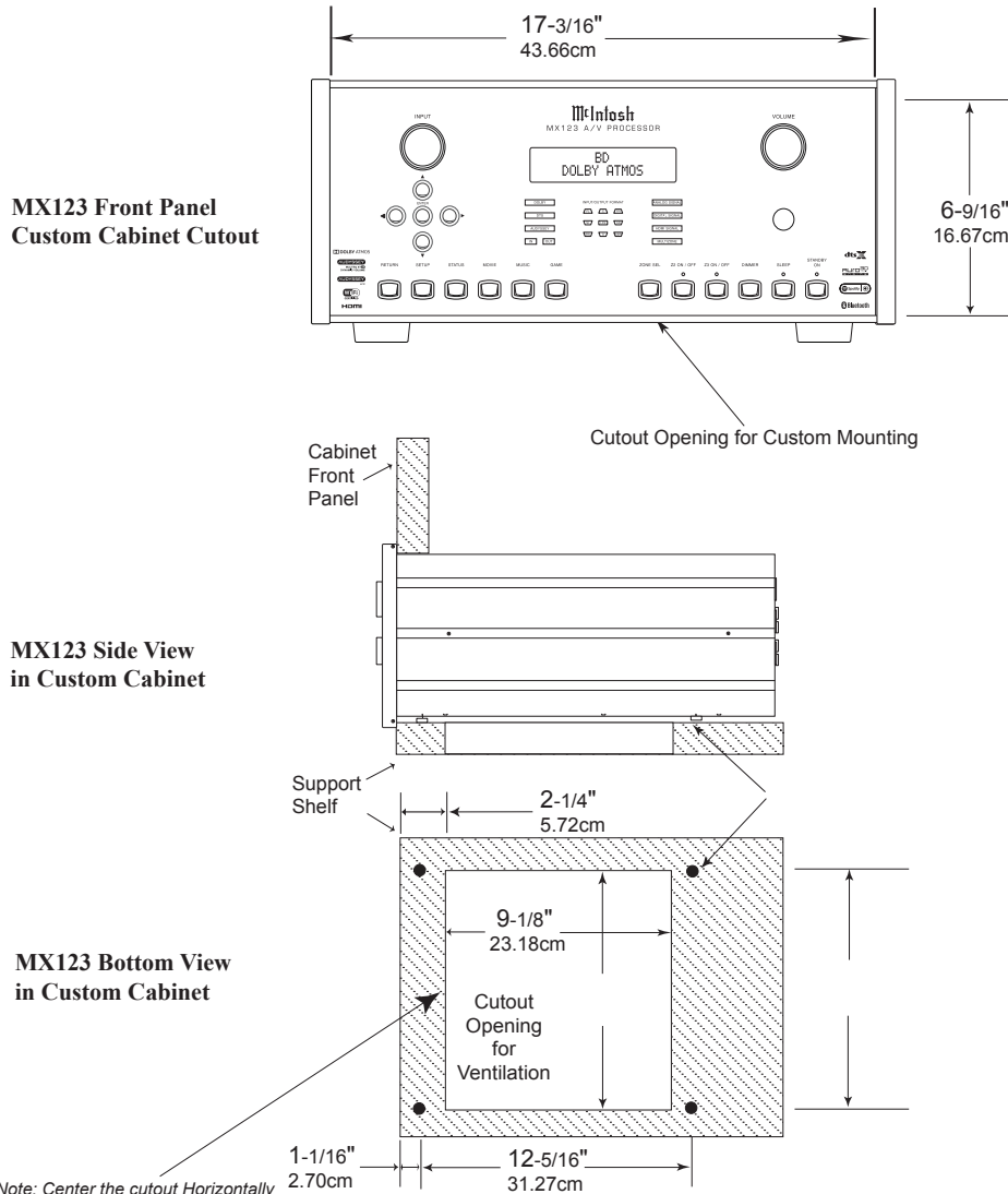
Figure 02– Custom cutout dimensions
