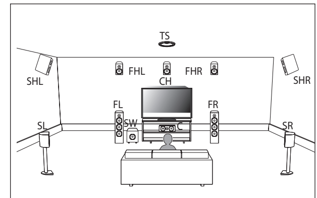
Figure 16– Auro-3D layout example
