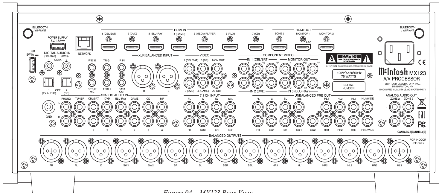
Figure 04– MX123 Rear View
