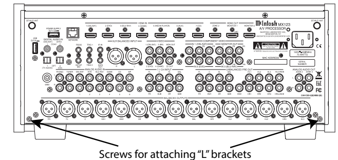
Figure 03– “L” bracket screws
