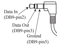
Figure 05— Mini plug for RS232 connection
