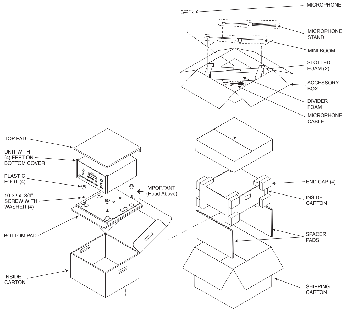
Figure 29– Re-packing diagram
